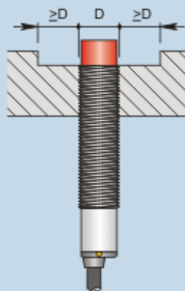
Non flush mounting
