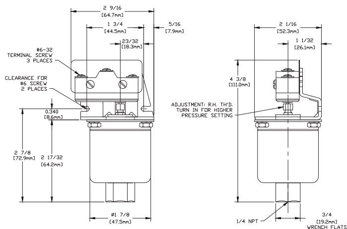
Type J54S Models 126 - 164
