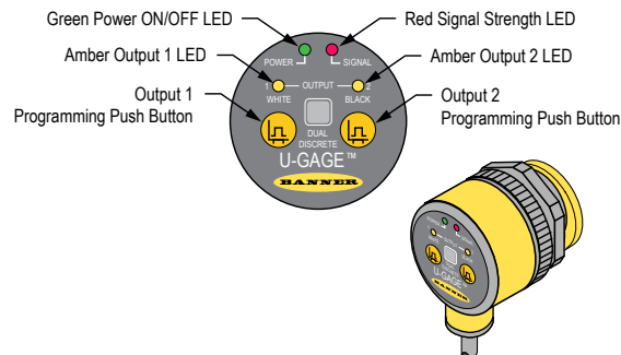
U-GAGE T30 Series sensor programming push buttons and indicators
