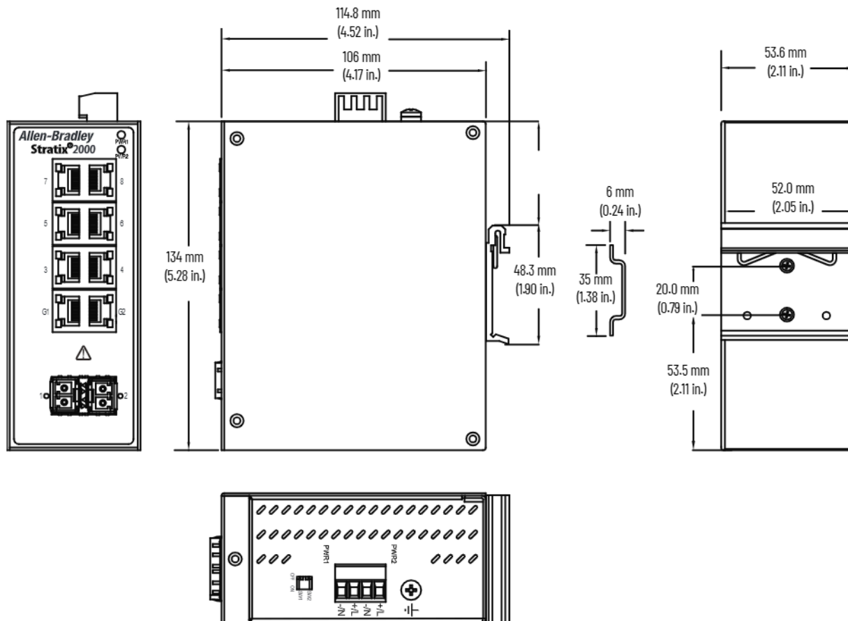
Figure 3 - 1783-US6T2T62F/B, 1783-US6T2T62H/B, 1783-US8T62GX/B
