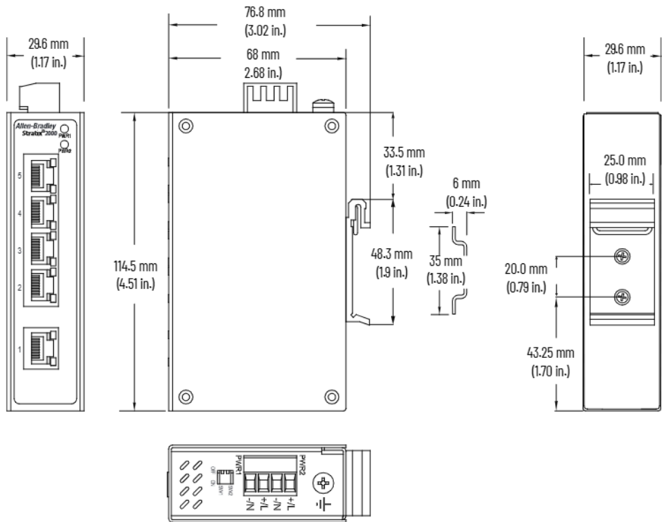
Figure 1 - 1783-US5T/B, 1783-US5TG/B, 1783-US4T1F/B, 1783-US4T1H/B
