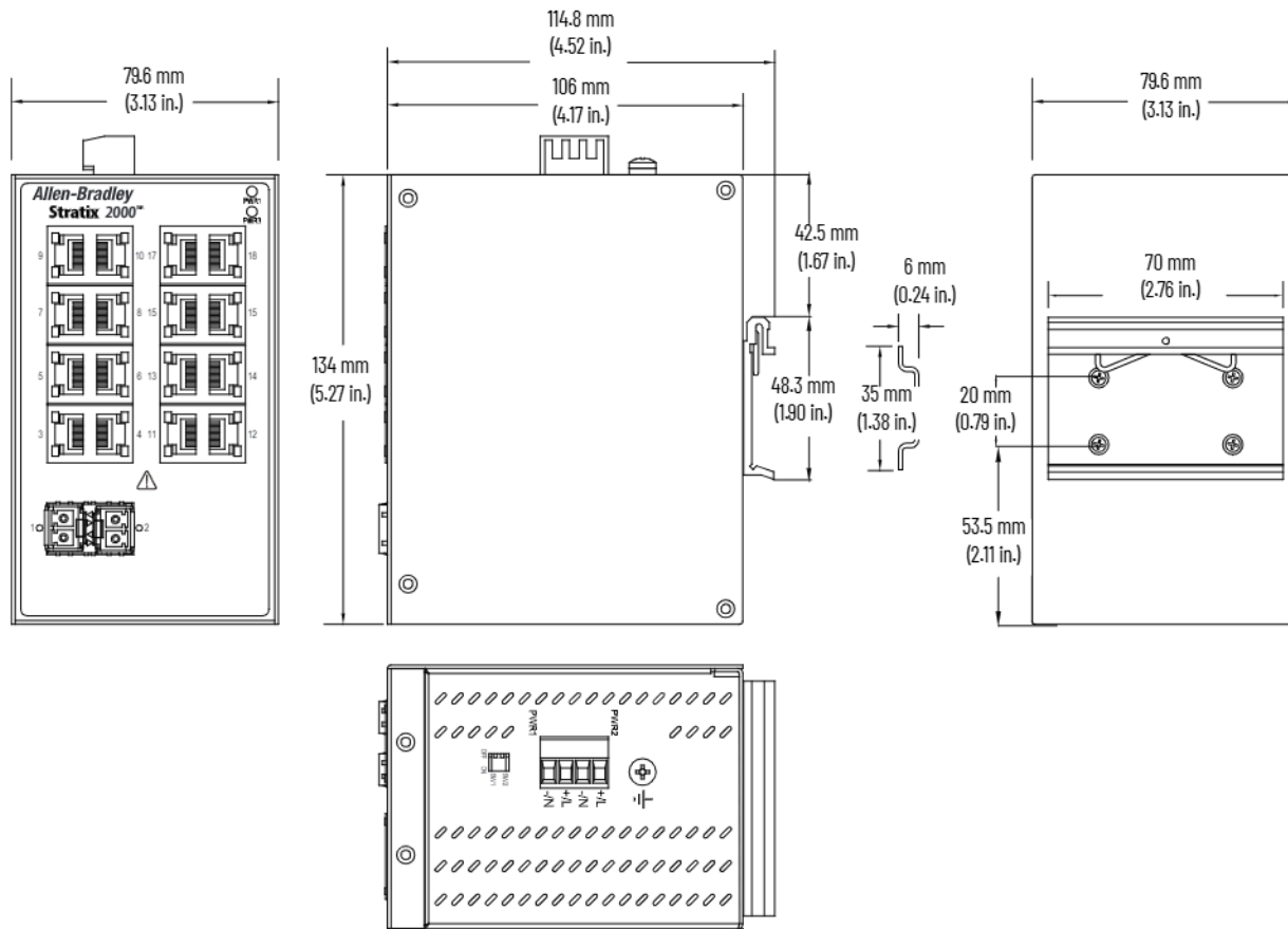
Figure 4 - 1783-US16T/B, 1783-US16T2S/B
