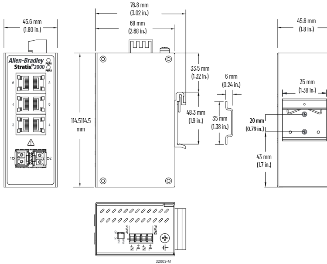
Figure 3 - 1783-US6T2T62F/B, 1783-US6T2T62H/B, 1783-US8T62GX/B
