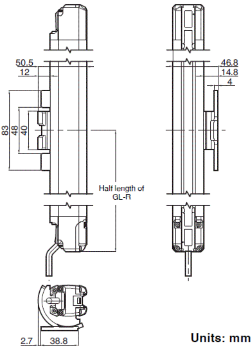
When mounted on GL-R (Side mounting)
