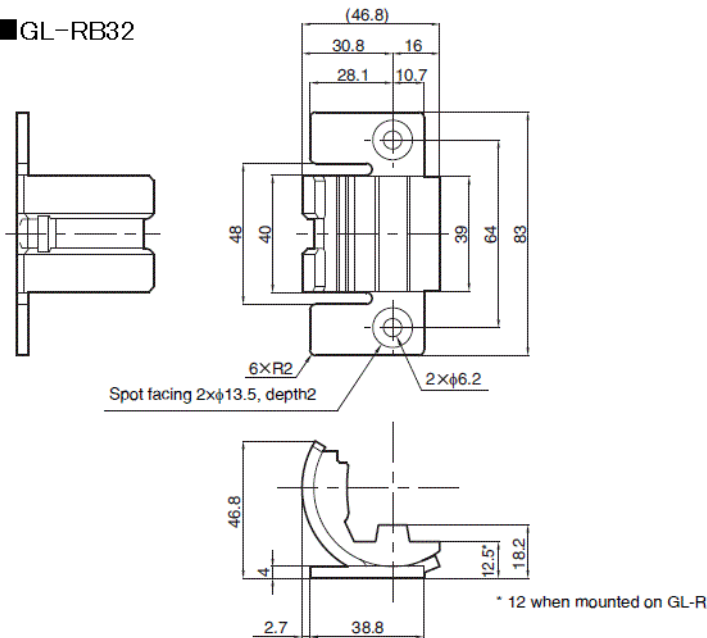
When mounted on GL-R (Back mounting)
