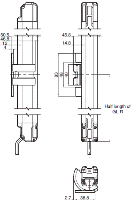
When mounted on GL-R (Back mounting)
