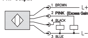
Diagram 4 PNP Output
