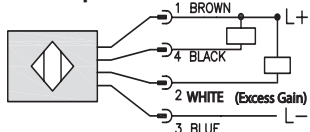
Diagram 1 NPN Output
