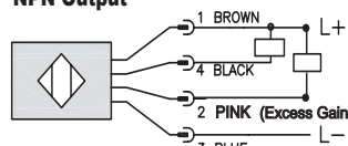
Diagram 3 NPN Output
