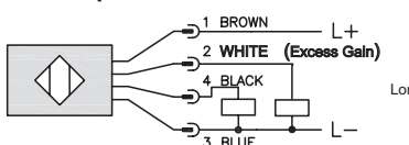
Diagram 2 PNP Output
